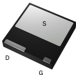
TPH3202LS 8x8 PQFN (bottom view)
