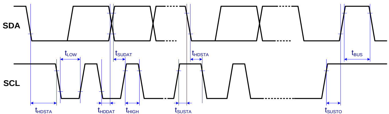
Figure 14. Bus Timing
