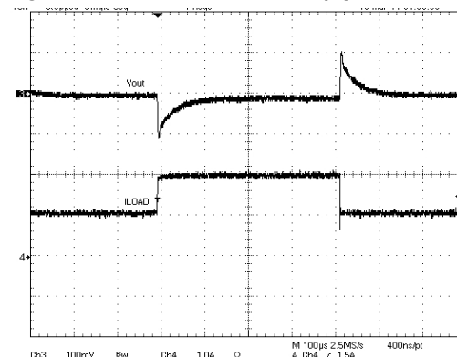
Figure 2.4 100mA to 1A Load Step ( V_{CC} = 12\text{V} , V_{OUT} = 3.3\text{V} )
