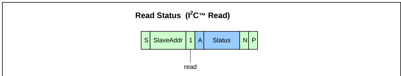
Figure 3.9 I 2 C™ Read Status
