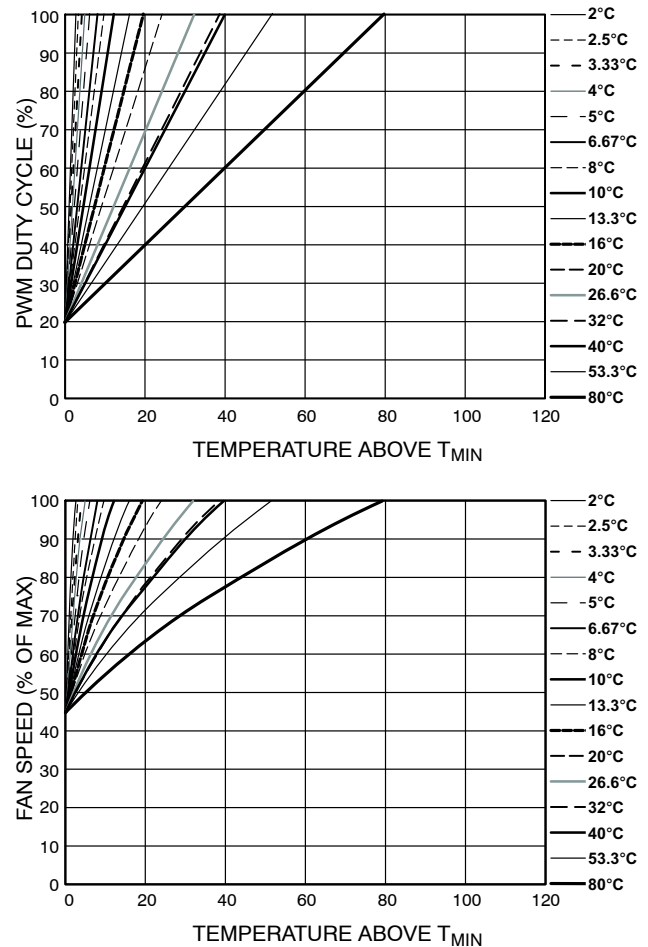
Figure 57. T_{\text{RANGE}} and % Fan Speed Slopes with \text{PWM}_{\text{MIN}} = 20\%
