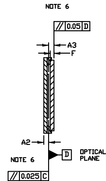
SECT. A-A
