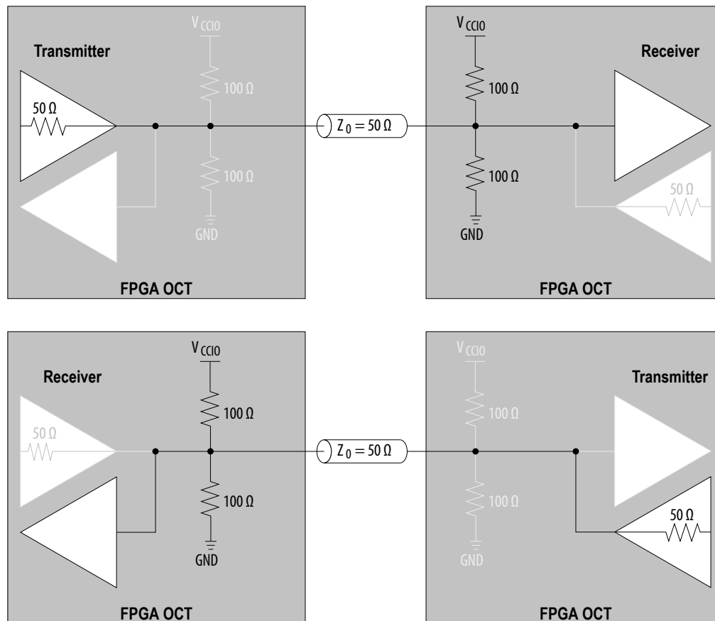
Figure 5-11: Dynamic R_T OCT in Arria V Devices
