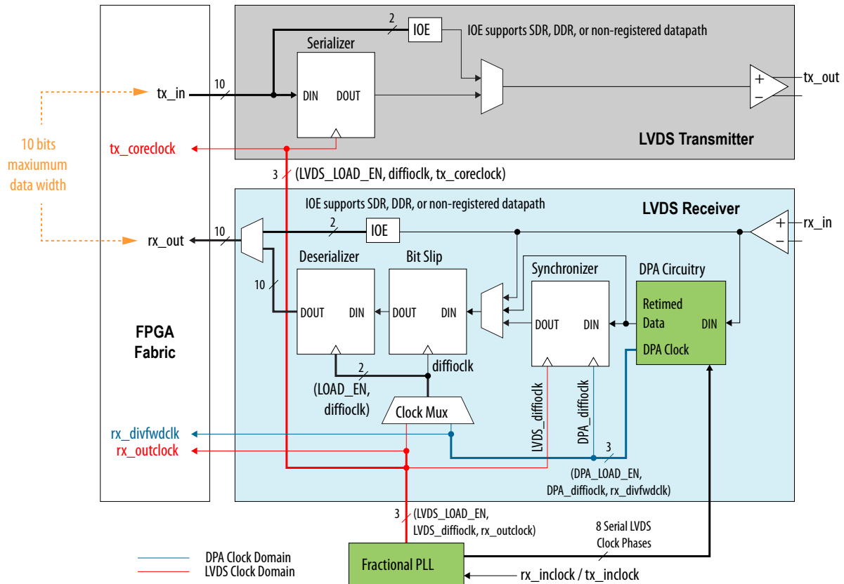
Figure 6-6: LVDS SERDES
