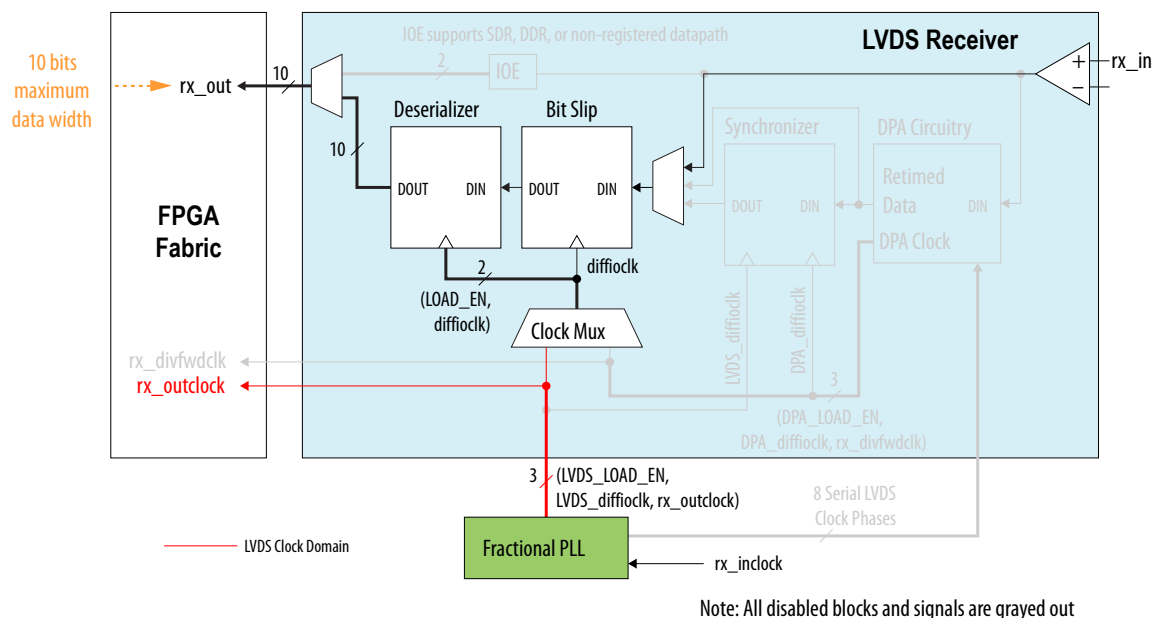
Figure 6-31: Receiver Data Path in Non-DPA Mode
