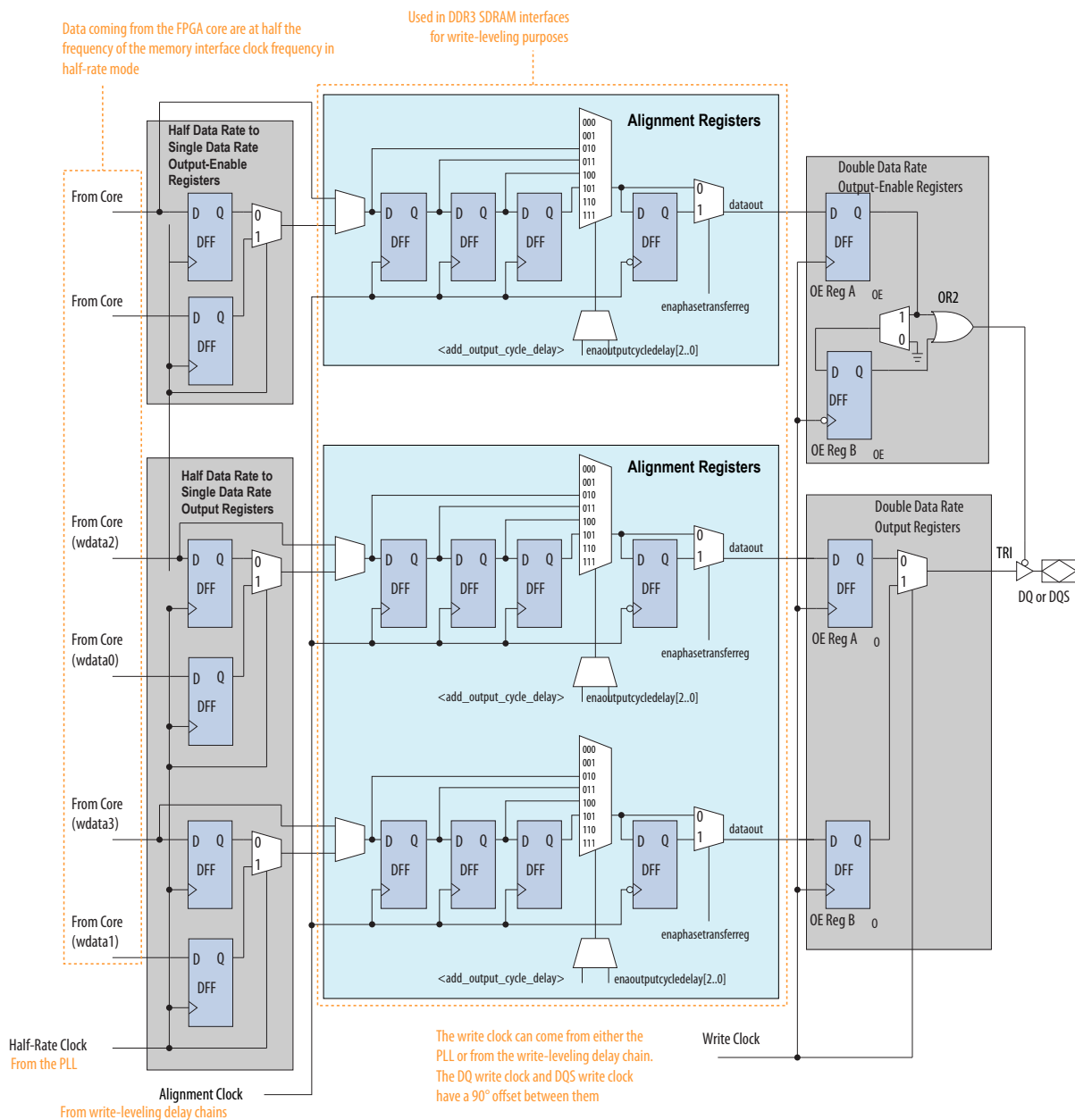
The following figure shows the registers available in the Arria V GZ output and output-enable paths. You can bypass each register block of the output and output-enable paths.
