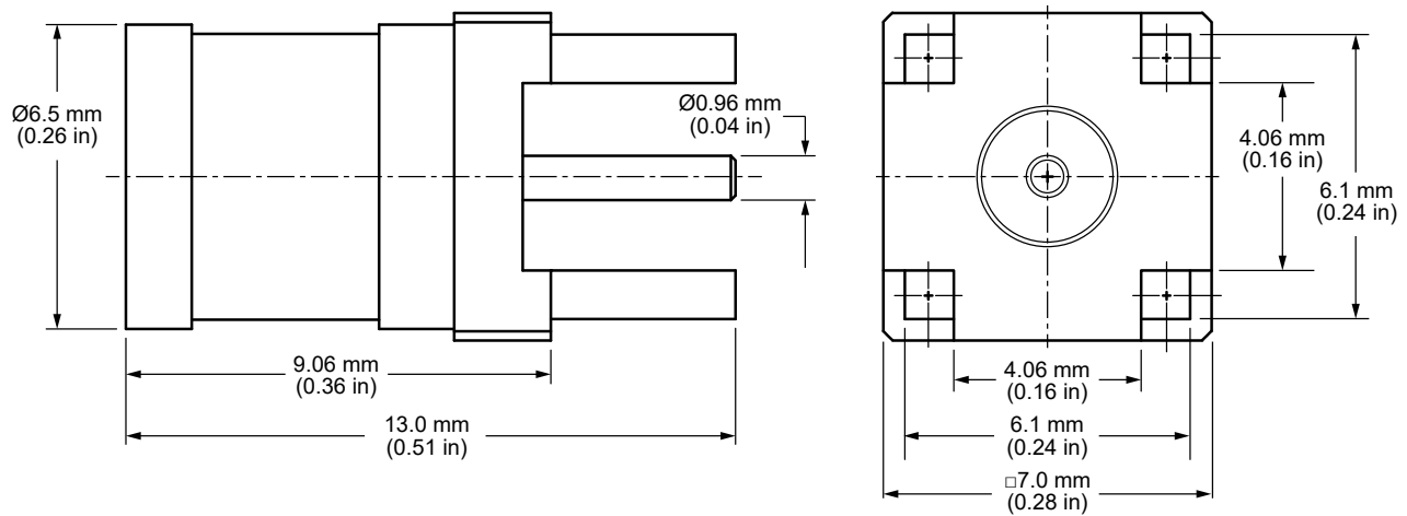
Figure 1. Product Dimensions for the CONSMB006-G Connector
