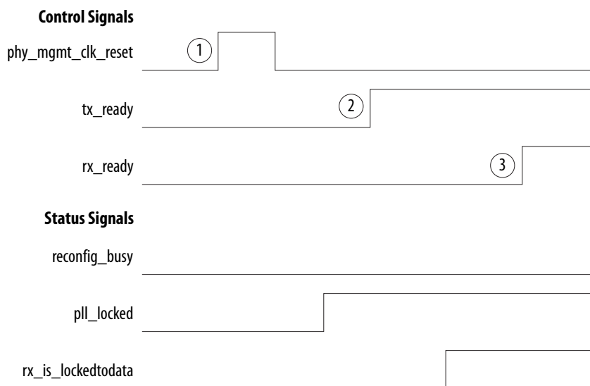
Figure 3-3: Reset Sequence Timing Diagram Using Embedded Reset Controller during Device Operation
