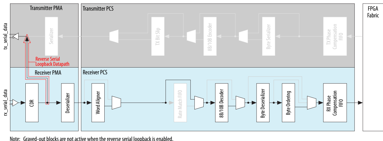
Figure 6-4: Reverse Serial Loopback Datapath
