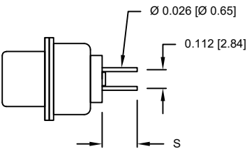
SIGNAL CONTACTS
