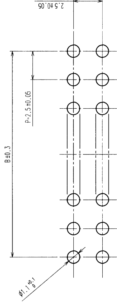
RECOMMENDED PATTERN ( 5 : 1 )
