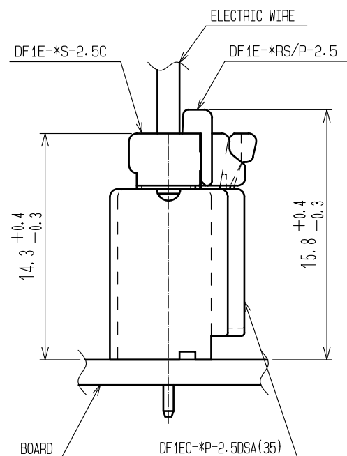
APPLICATION DIAGRAM(3:1)
