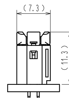
MATING FIGURE (2:1)
