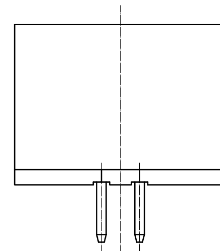
MATING FIGURE (2:1)
