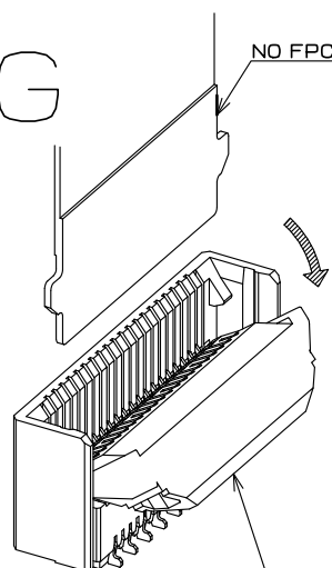
Before mounting
