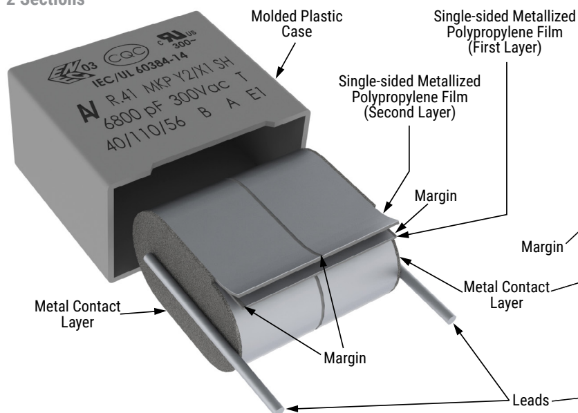
2 Sections
