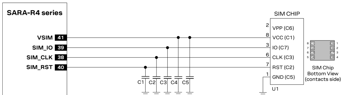
Figure 52: Application circuits for the connection to a single Surface-Mounted SIM chip, with SIM detection not implemented
