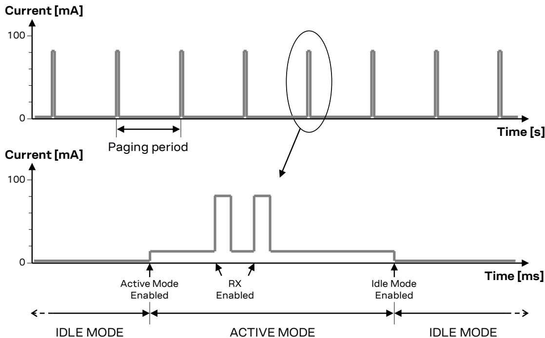
Figure 14: Example of VCC current consumption profile with low power mode enabled (AT+UPSV≠0), module registered with the network: the module is in low-power idle mode, with no concurrent activities executed, and it periodically wakes up to active mode for paging block reception
