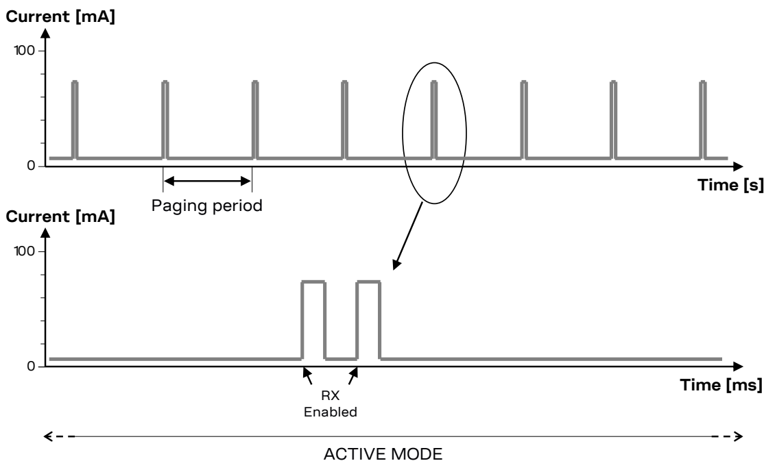
Figure 15: Example of VCC current consumption profile with low power mode disabled (AT+UPSV=0), module registered with the network: active mode is held, the receiver is periodically temporarily activated for paging block reception
