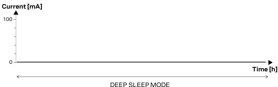
Figure 13: Example of VCC current consumption profile in ultra low power deep sleep mode with the use of the PSM enabled (AT+CPSMS \neq 0), module registered with the network: the module is in ultra low power deep sleep mode, with no concurrent activities executed, and it does not periodically wake up for paging block reception, but it wakes up upon the expiration of the periodic update timer set by the network or due to proper toggling of the PWR_ON / PWR_CTRL input line
