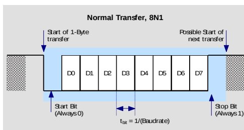
Figure 20: Description of UART 8N1 frame format (8 data bits, no parity, 1 stop bit)
