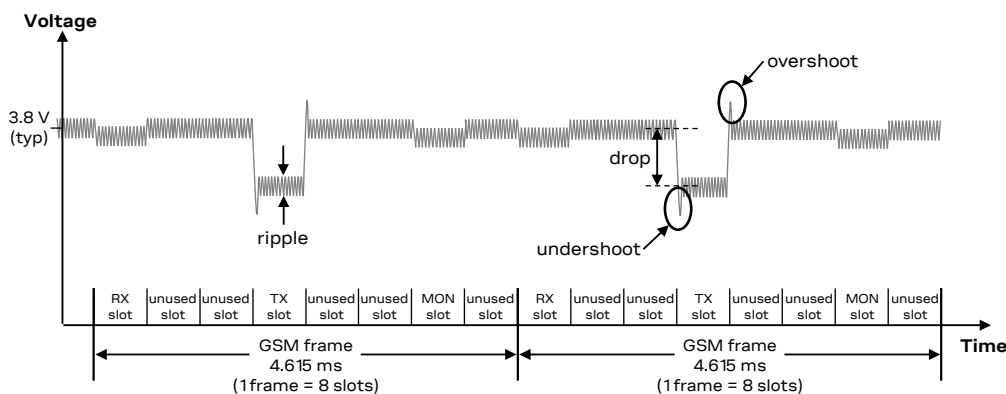
Figure 11: Description of the VCC voltage profile versus time during a 2G single-slot call (1 TX slot, 1 RX slot)
