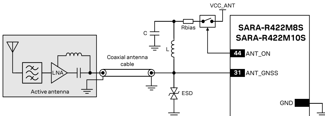
Figure 44: Typical circuit with active antenna connected to GNSS RF interface, using an external supply
