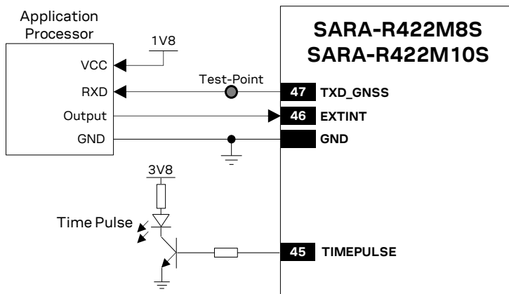
Figure 69: Application circuit for GNSS peripheral input output
