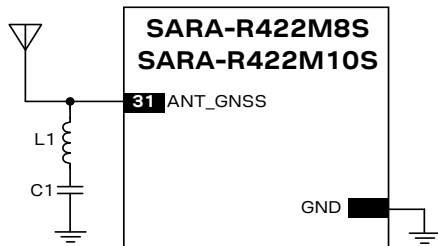
Figure 46: Simple notch filter for improved in-band jamming immunity against a single jamming frequency
