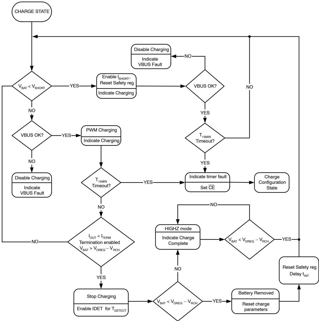
Figure 36. Charge Mode
