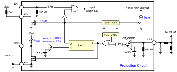
Figure 42. Over-Current Protection
