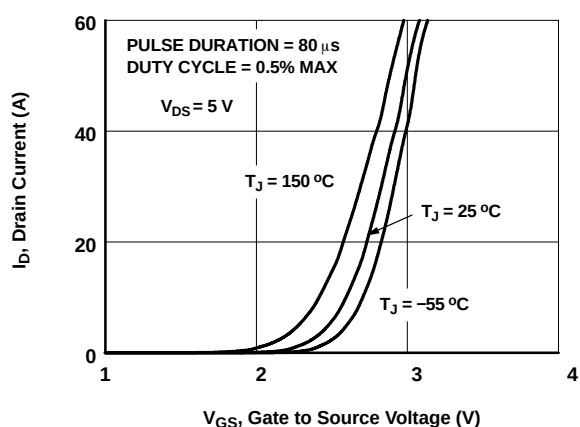
Figure 18. Transfer Characteristics
