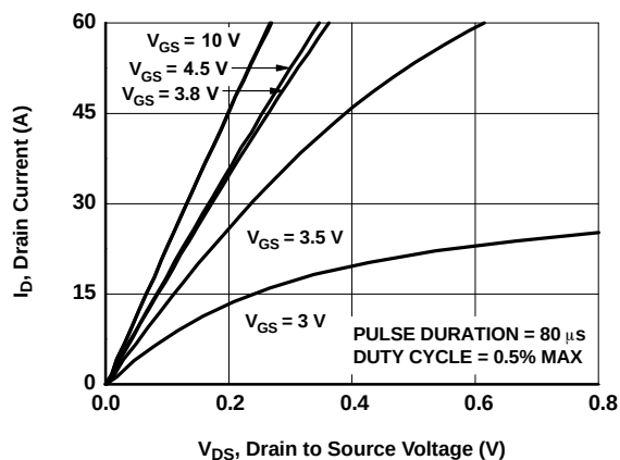
Figure 14. On-Region Characteristics
