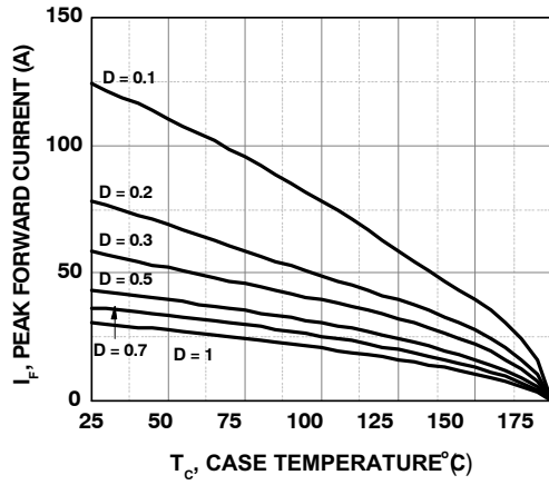
Figure 3. Current Derating
