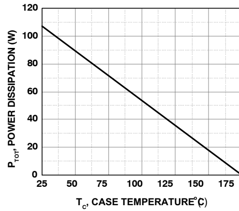
Figure 4. Power Derating
