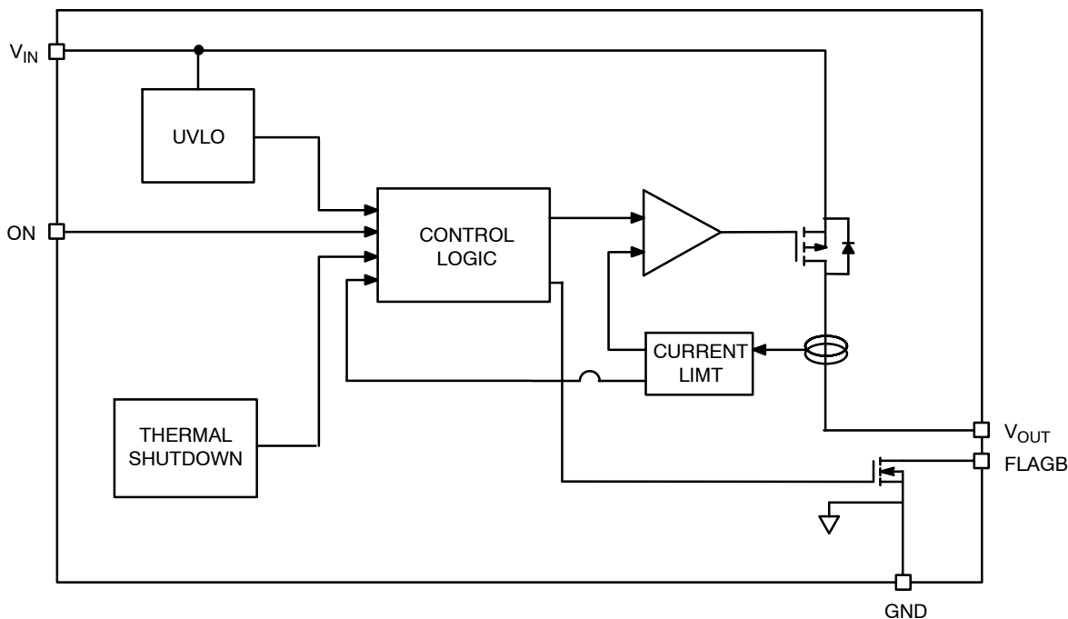
Figure 2. Block Diagram
