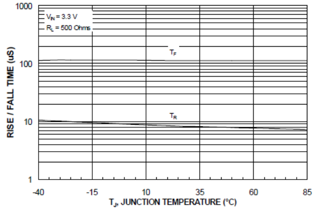
Figure 11. T_{RISE} / T_{FALL} vs. Temperature
