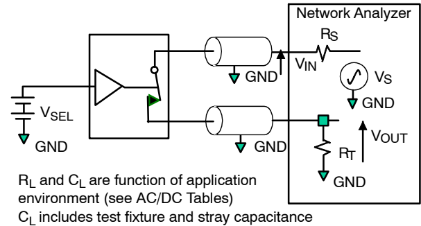
Figure 19. Total Harmonic Distortion (THD + N)
