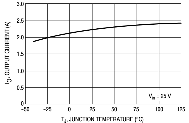
Figure 5. Current Limit
