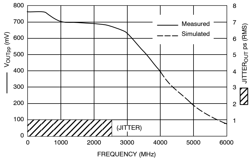
Figure 2. F_{max}/Jitter
