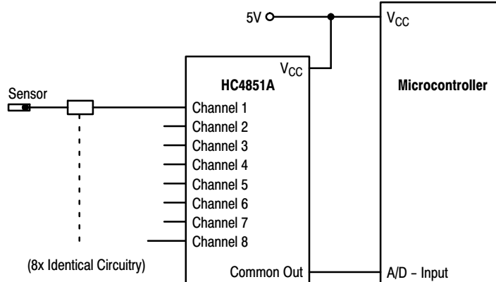
Figure 12. MC74HC4851A Solution
