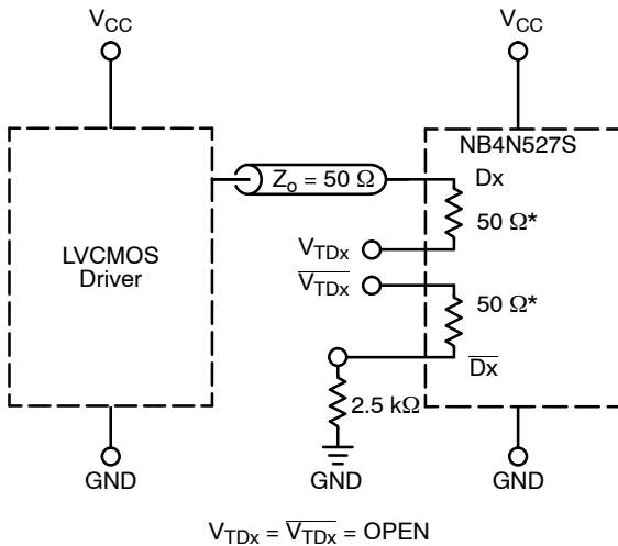
Figure 11. LVC MOS Interface
