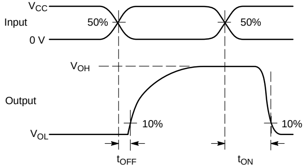
Figure 15. t_{ON}/t_{OFF}
