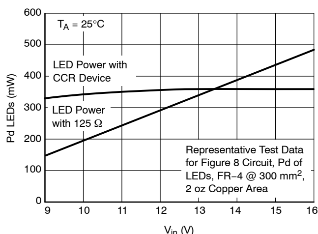
Figure 11. LED Power
