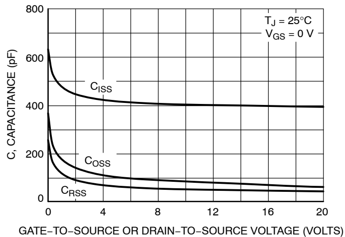
Figure 22. Capacitance Variation
