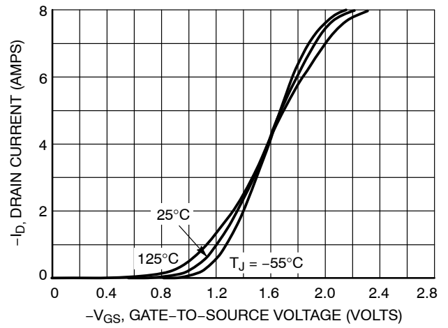
Figure 13. Transfer Characteristics
