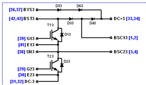
Figure 1. NXH300B100H4Q2F2PG/SG/SG-R Schematic Diagram
