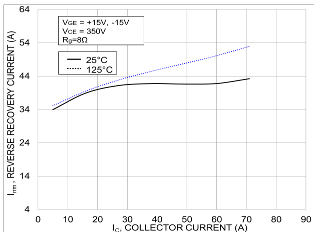
Figure 34. Typical Reverse Recovery Current vs. I_C
