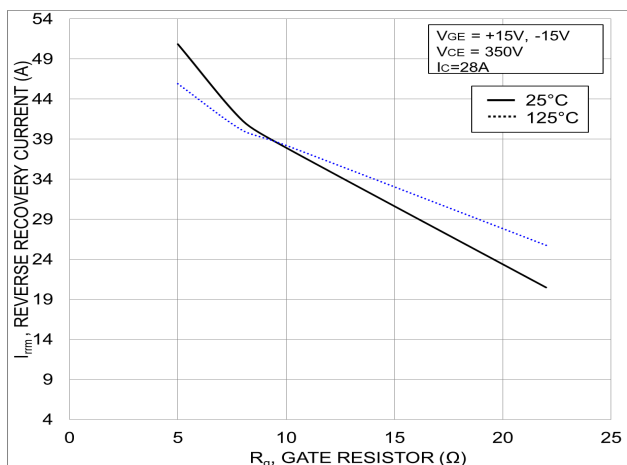
Figure 30. Typical Reverse Recovery Peak Current vs. R_g
