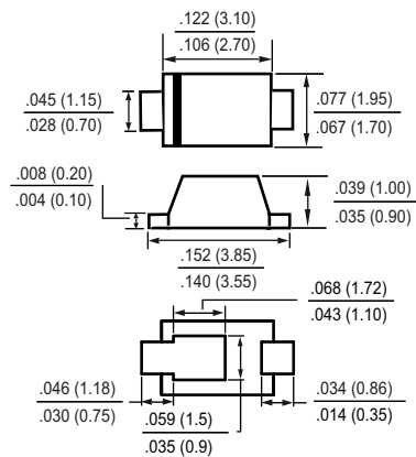
SOD-123FL
