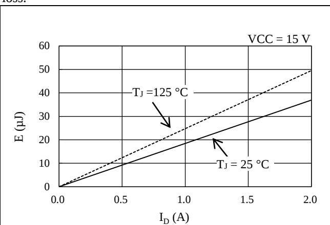
Figure 14-14. Low-side Switching Loss
