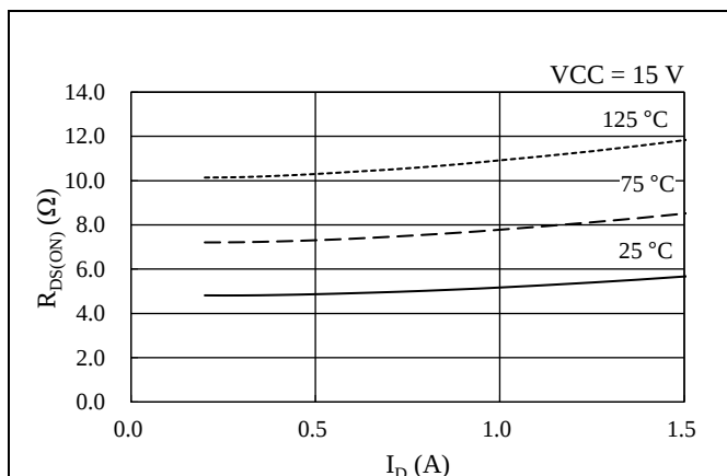
Figure 14-9. Power MOSFET R_{DS(ON)} vs. I_D
