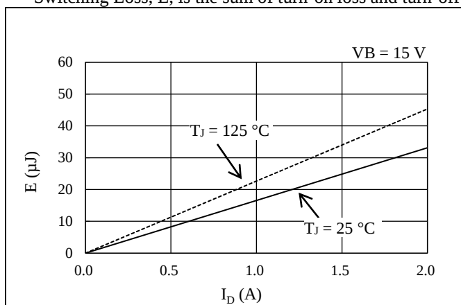
Figure 14-13. High-side Switching Loss
