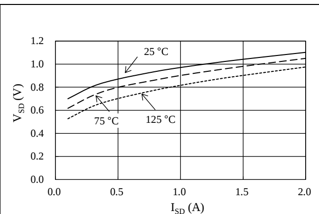
Figure 14-12. Power MOSFET V_{SD} vs. I_{SD}
