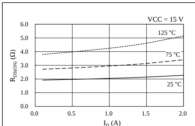
Figure 14-11. Power MOSFET R_{DS(ON)} vs. I_D
